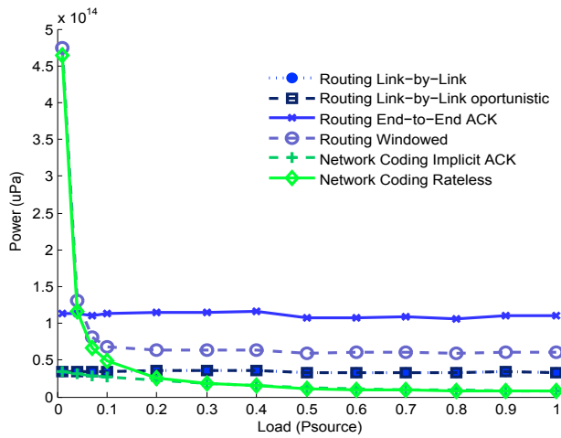
Figure 7: Average power consumed by node vs load for a 6 node network, transmitting 10 packets using optimal power calculation
