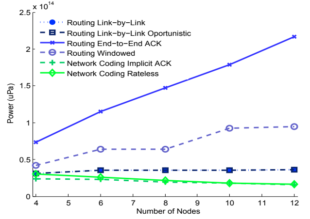
Figure 10: Average power consumed by node vs total number of nodes in the network, transmitting 10 packets generated with P_{source} = 0.2 using optimal power calculation
