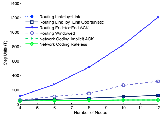
Figure 15: Average number of steps vs number of nodes in network, transmitting 10 packets using fixed power in all nodes and P_{source} = 0.2
