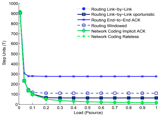
Figure 13: Average number of steps vs load for a 6 node network, transmitting 10 packets using fixed power in all nodes
