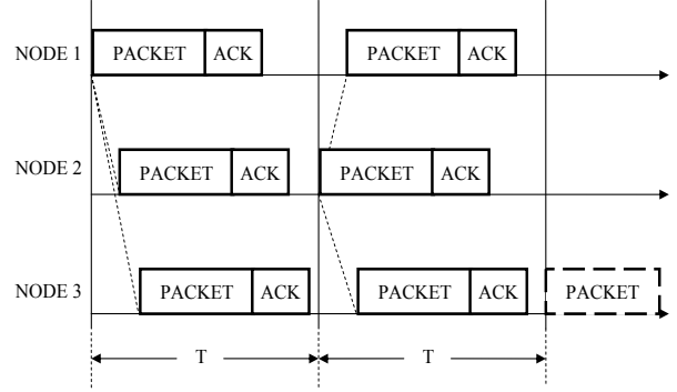
Figure 5: MAC layer.
