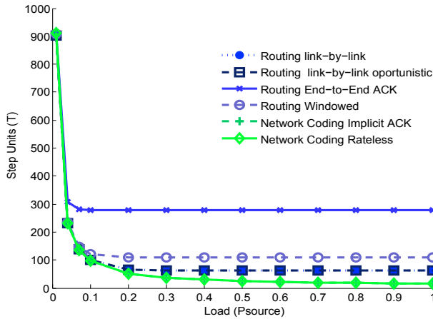
Figure 6: Average number of steps vs load for a 6 node network, transmitting 10 packets using optimal power calculation
