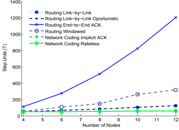
Figure 9: Average number of steps vs total number of nodes in the network, transmitting 10 packets generated with P_{source} = 0.2 using optimal power calculation
